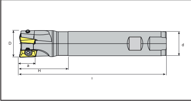
AX.T12 AX.T17 SUMITOMO
